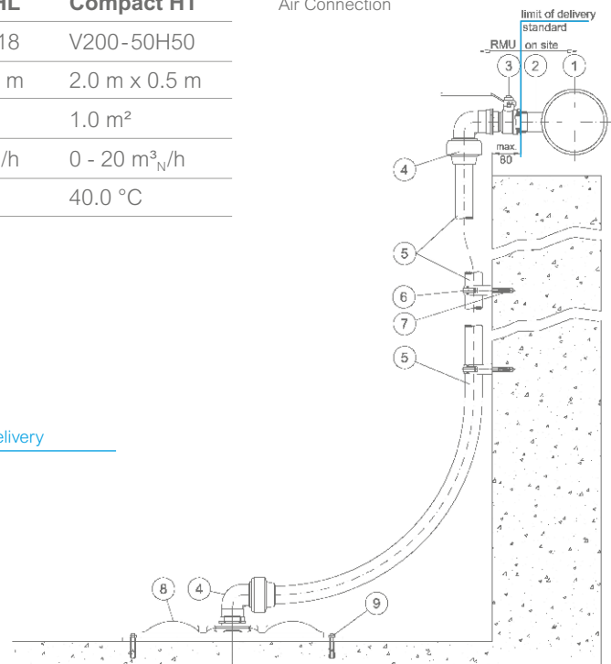
Air Connection
